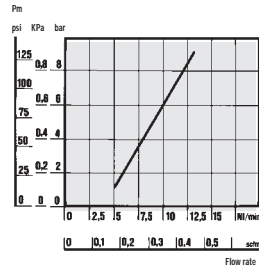
MINIMUM OPERATING FLOW CHART
